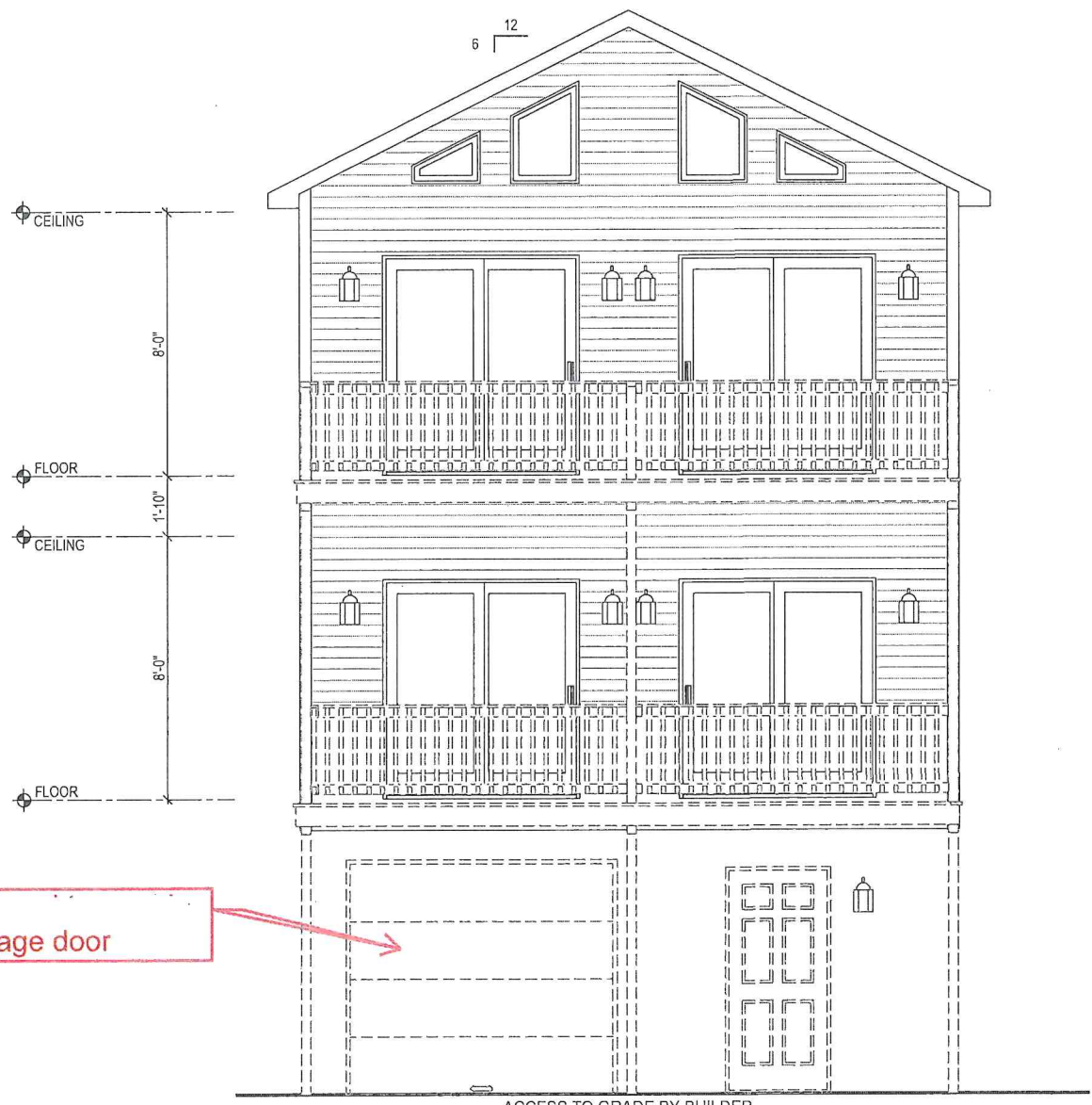
FRONT ELEVATION
