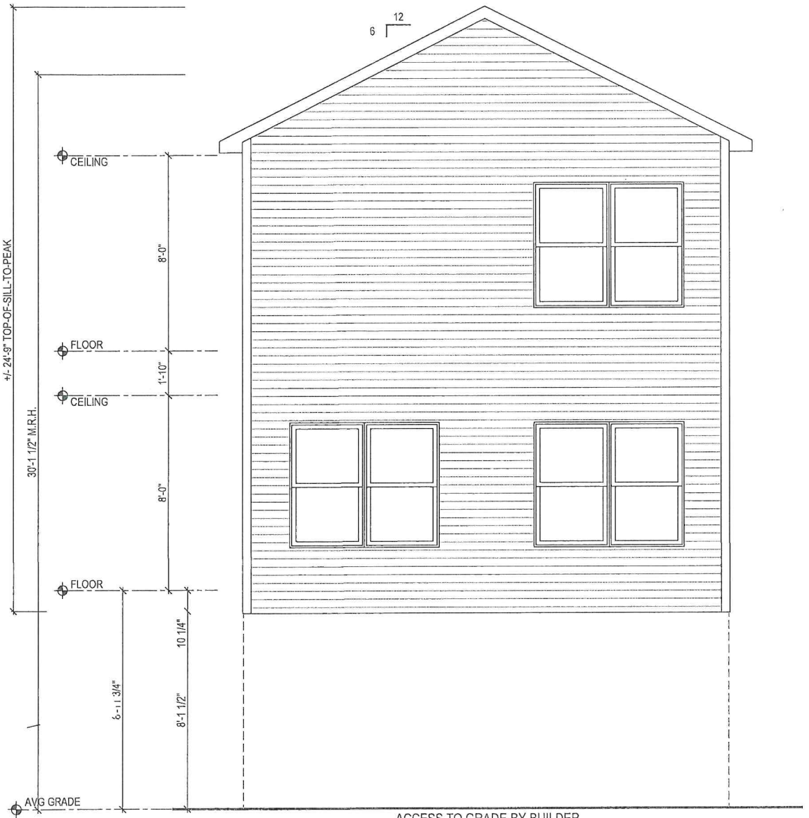
REAR ELEVATION
